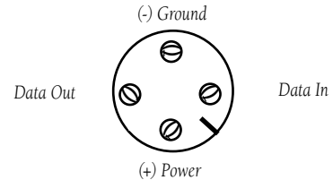
Cable Plug End View
